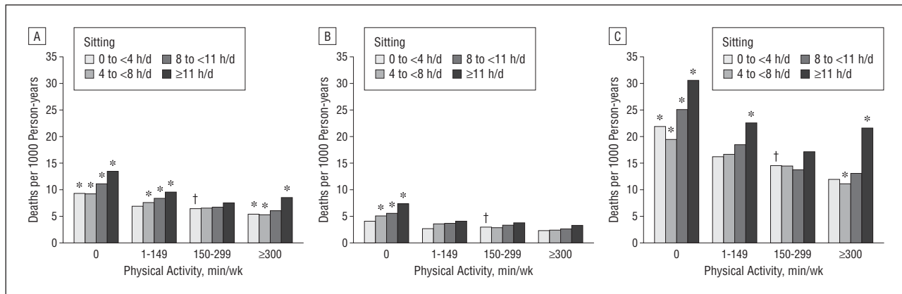
Figure. The combined relationships of sitting and physical activity with all-cause mortality. A, All participants ( n=222\,497 ). B, Healthy participants who at baseline had no cardiovascular disease, diabetes mellitus, or cancer, with the exception of nonmelanoma skin cancer ( n=145\,713 ). C, Participants with cardiovascular disease or diabetes at baseline ( n=52\,229 ). Deaths per 1000 person-years were adjusted for sex, age, educational level, marital status, urban or rural residence, body mass index, smoking status, self-rated health, and receiving help with daily tasks for a long-term illness or disability. * P < .05 compared with the reference group. †Reference group.
